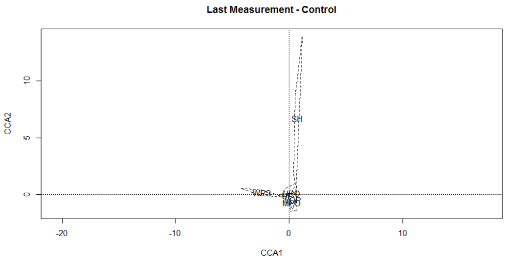
Figure 6d. Seedlings – Control at last measurement. Convex hull separates vegetation types by sandhill (SH), upland (UP), upperslope pine oak (UPO), midslope oak pine (MPO), lowerslope pine hardwood (LPO), and wetland pine savanna (WPS).
