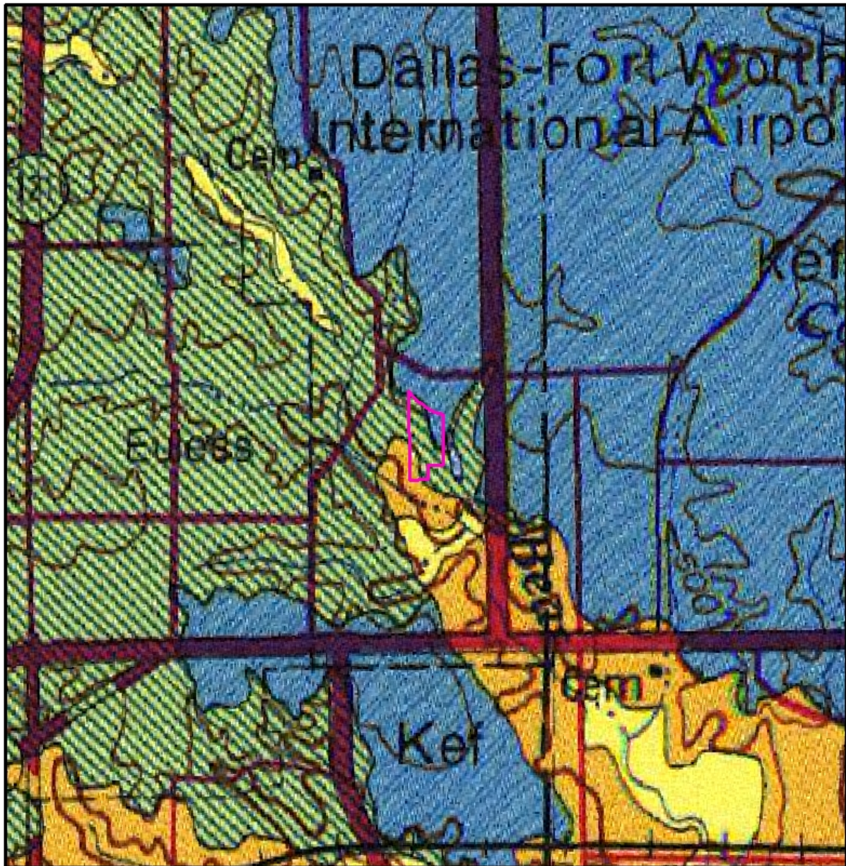
Figure 2.1 Geologic Setting
