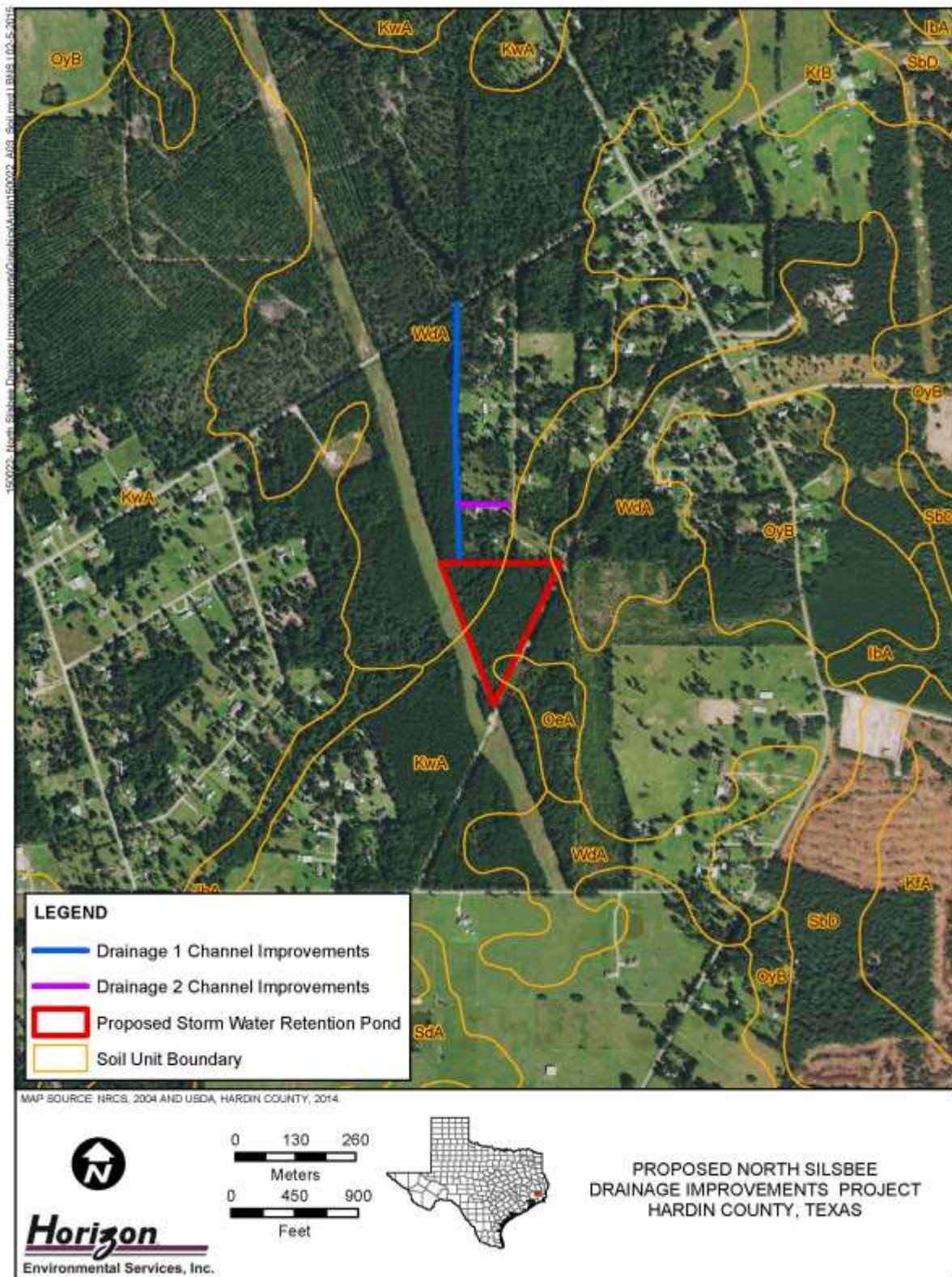
Figure 3. Distribution of Soils Mapped with APE
