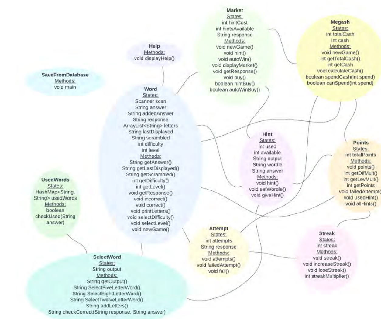
Figure 1 A graph displaying the methods for the terminal-based solution
