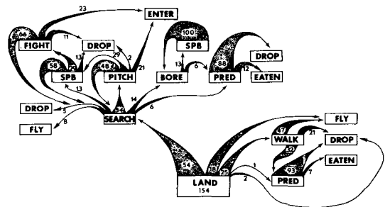
FIG. 1. —Behavioral sequence flow diagram for SPB behavior on the bark of host trees. Percentage of beetles within a behavior category that proceed to another are indicated (n = 154).
