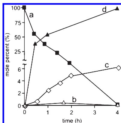
Figure 7. Reaction profile of fiber optic delivering light and oxygen to the probe tip (a) percent sensitizer bioconjugate 1 , (b) percent surface-bound dioxetane 2 , (c) percent 3 photoreleased into toluene- d_8 at room temperature, and (d) percent 3 photoreleased into petrolatum at 65 °C.
