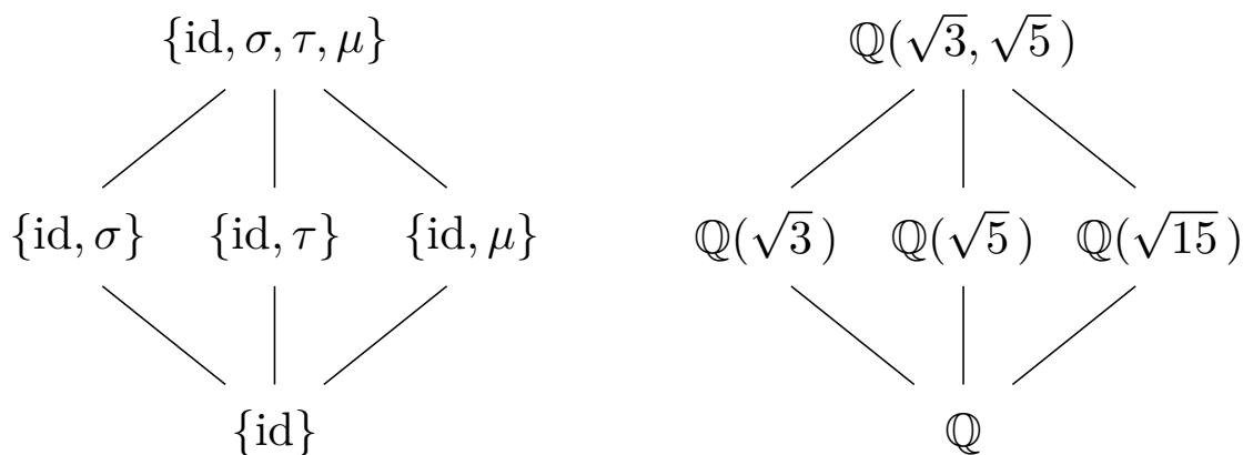
Figure 23.22 G(\mathbb{Q}(\sqrt{3}, \sqrt{5})/\mathbb{Q})
