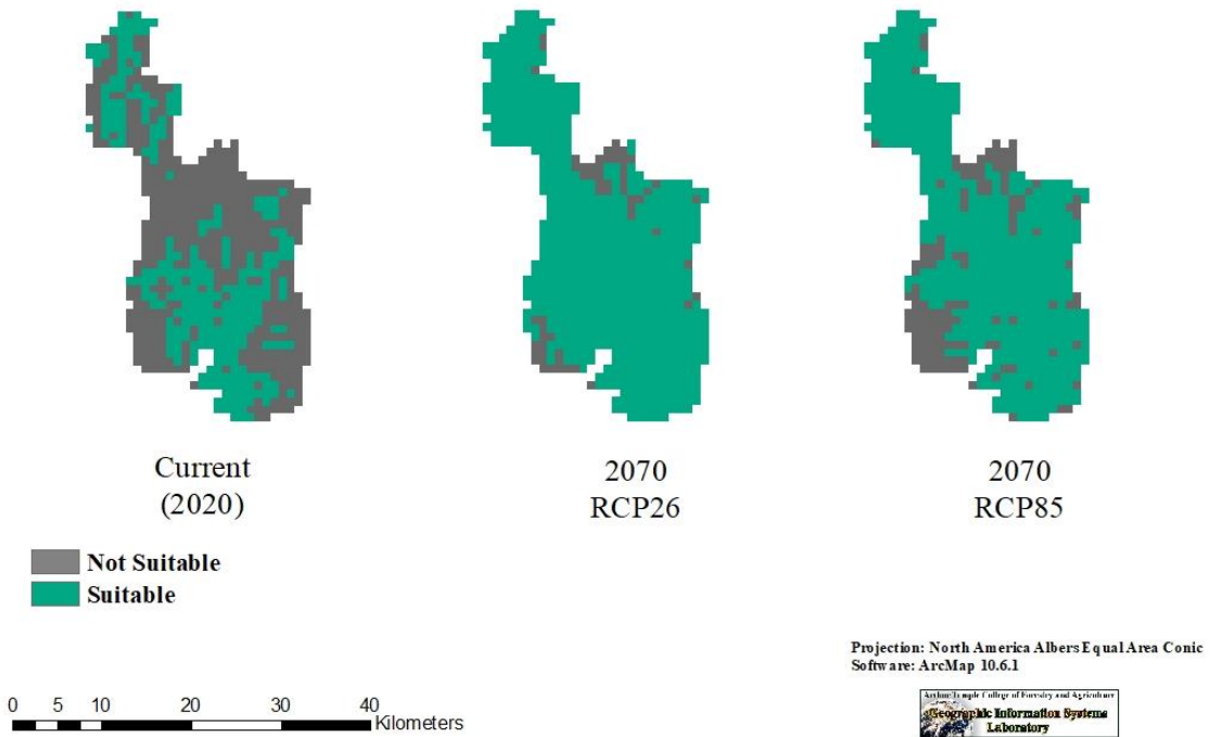
Figure 31. Forecasting SDM of C. humilis var. jonesii in ZION for the current year (2020) and 2070 using binary distribution of suitable versus not suitable habitat. The ‘10 percentile training presence’ threshold was calculated by MaxEnt to delineate suitable habitat in this analysis.
