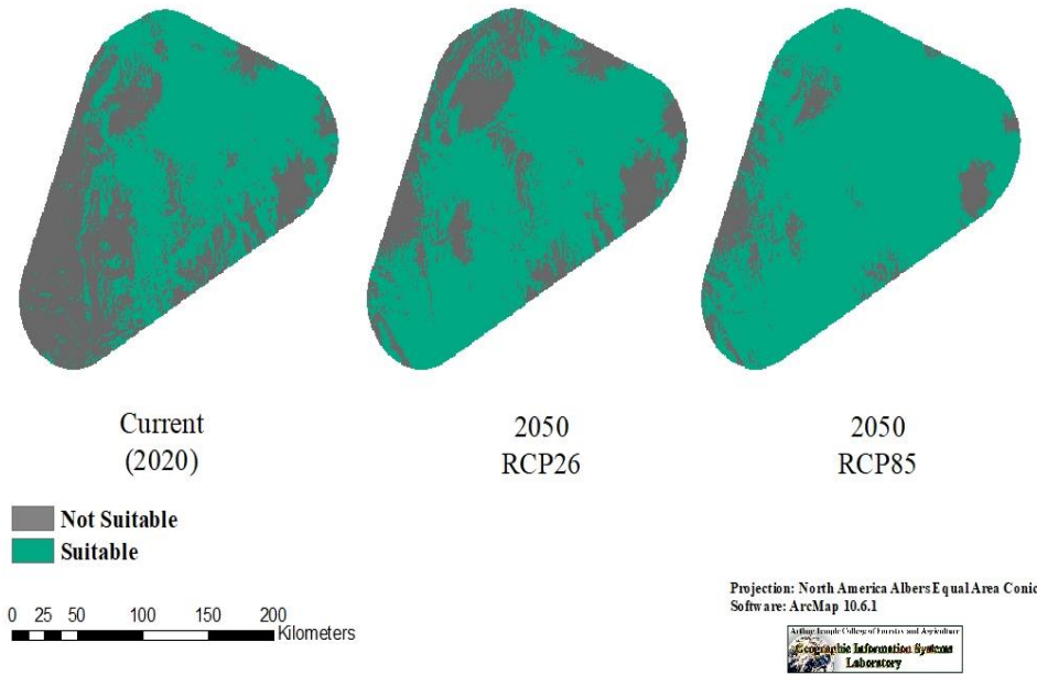
Figure 28. Forecasting SDM of C. humilis var. jonesii contrasting the suitable habitat for future climate scenarios for representative concentration pathways that describe greenhouse gas concentration of 2.6 W/m 2 and 8.5 W/m 2 for the year 2050. The SDM covers the complete training extent of the plant to better understand changes in suitable future habitat (see Figure 15). The ‘10 percentile training presence’ calculated by the MaxEnt output was used to delineate suitable habitat in this analysis.
